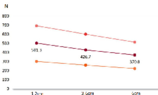
FY-RAF56N-40-B (OPEN)
