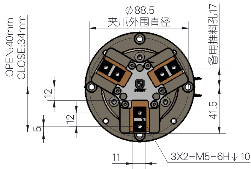
FY-RAF56N-40-B (CLOSE)
